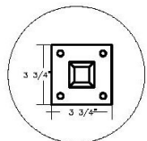
FLUSH MOUNT
